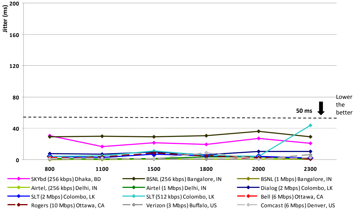
Fixed Broadband - Jitter ix and Packet Loss x Figure 5 - Jitter when pinged to International
