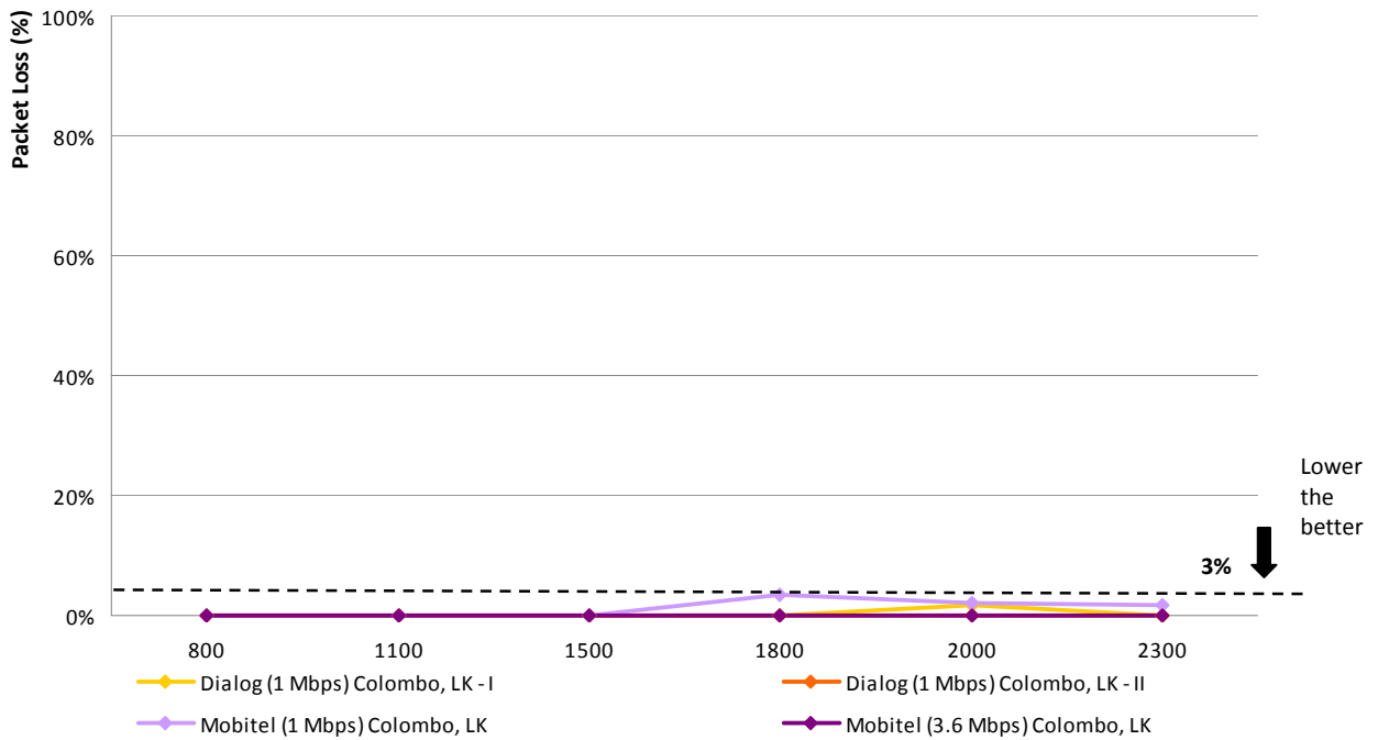
Figure 13 - Packet loss when pinged to International
